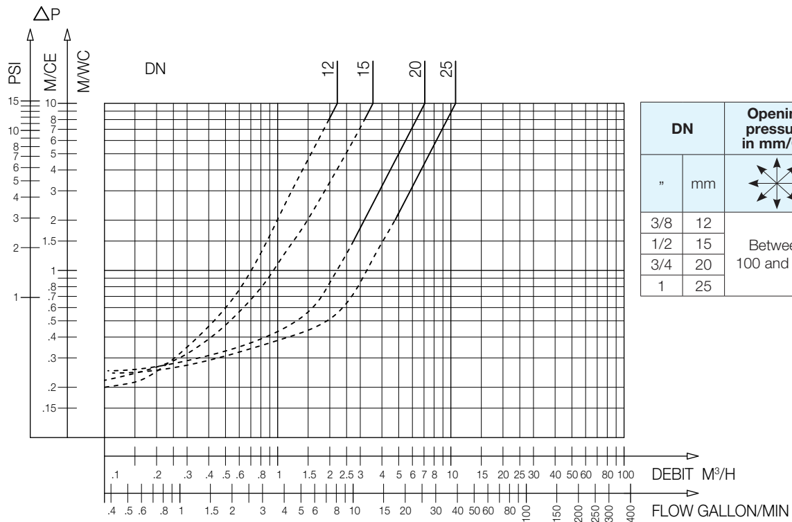
297 D - Headloss chart
